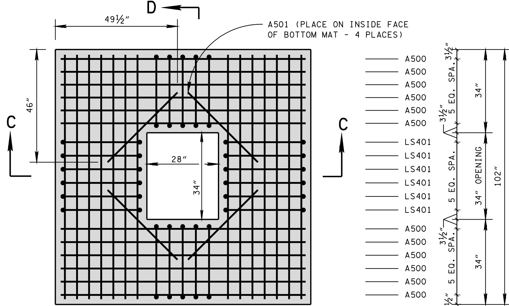
PLAN VIEW
