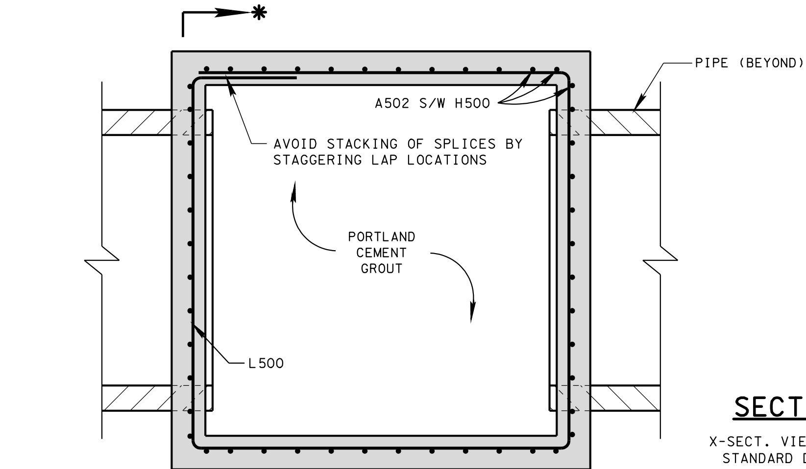
SECTION E-E
