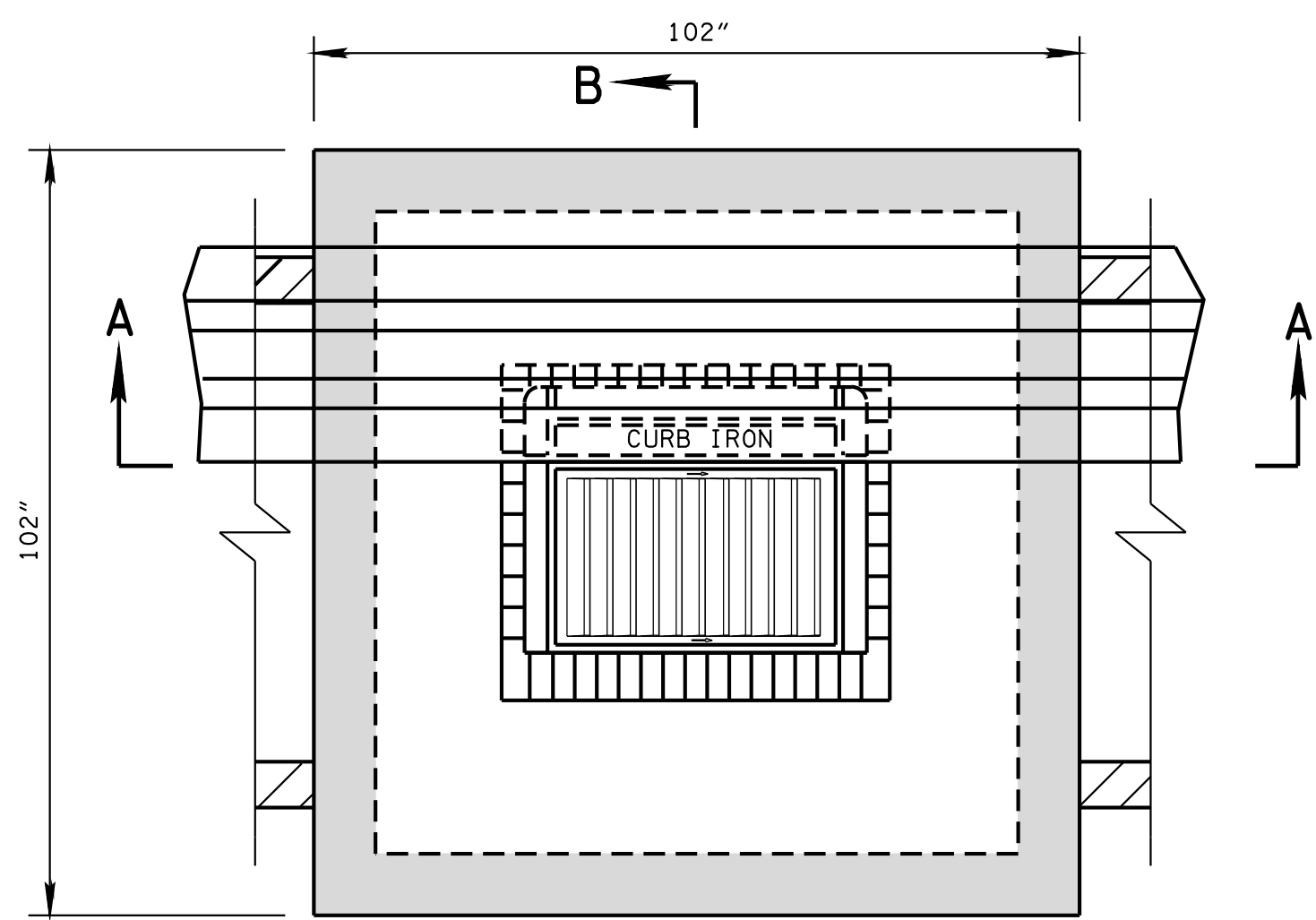
PLAN VIEW
