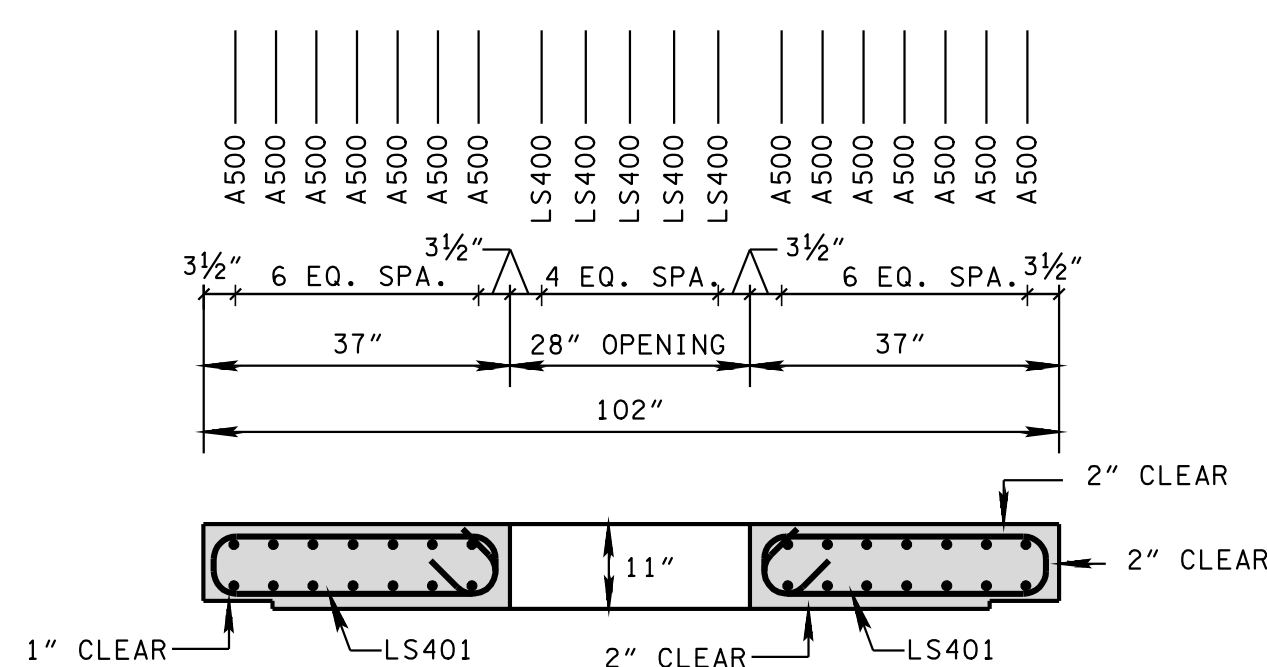
SECTION C-C
